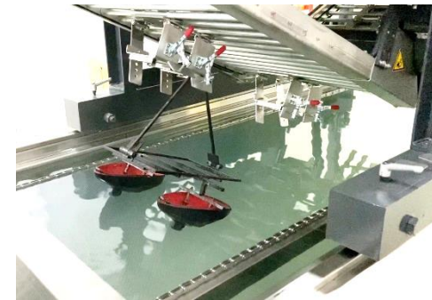
Fixture
